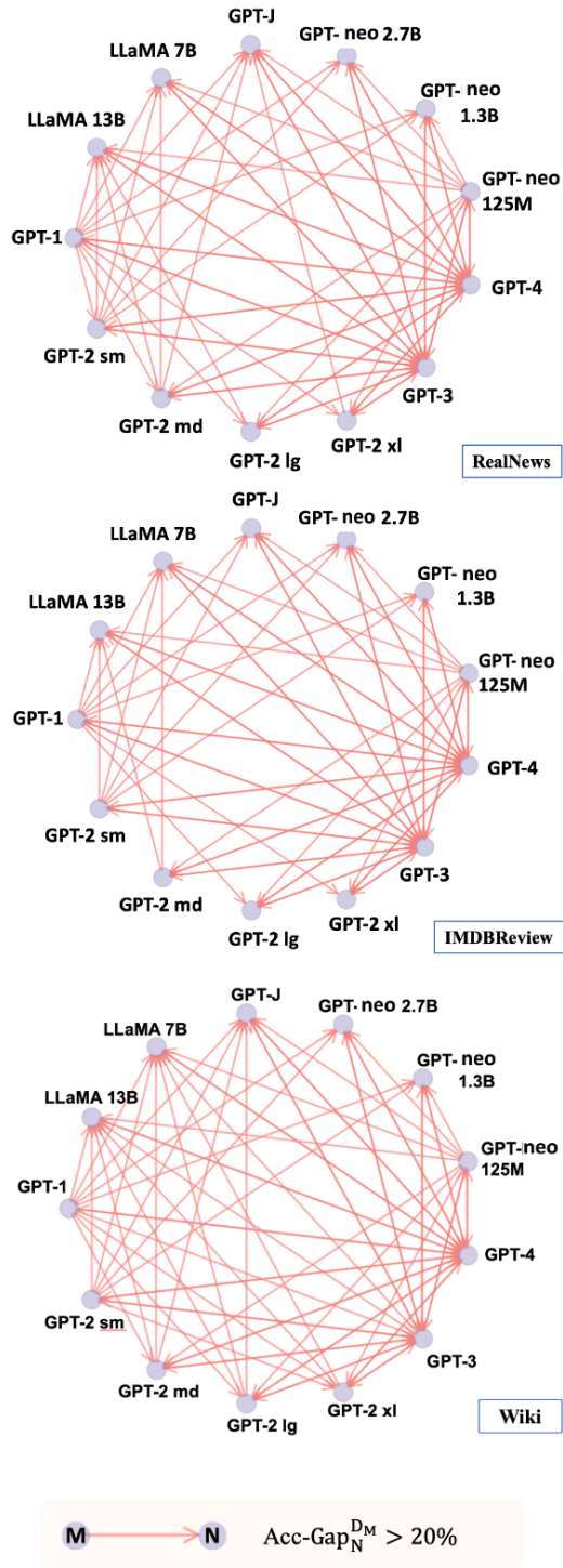
Figure 2: Detector-generator pairs with large (>20%) accuracy gap.
