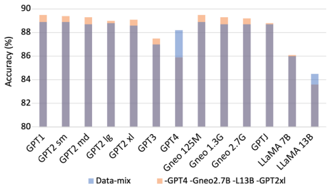
Figure 3: Accuracy comparison on each generator before and after pruning out four large-version LLMs on the RealNews dataset.
